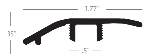
REDUCER
