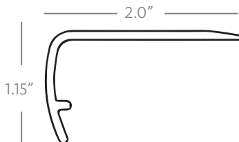
STAIR NOSE
