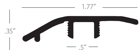
REDUCER
