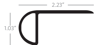
STAIR NOSE
