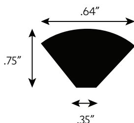
QUARTER ROUND
