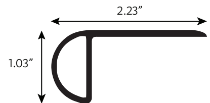
STAIR NOSE
