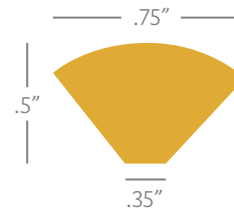
STAIR NOSE
