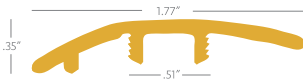
REDUCER
