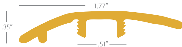
REDUCER
